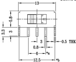
Outline Drawing
