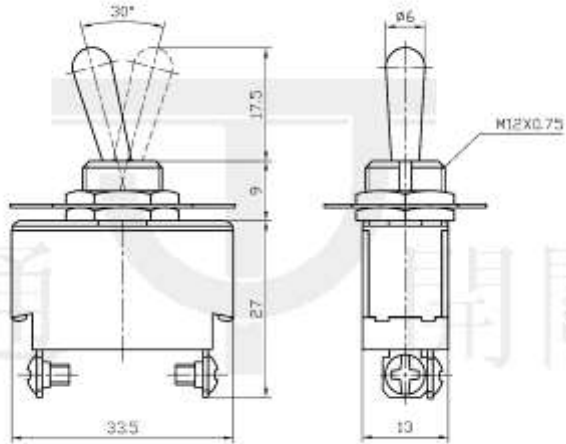
Mounting
