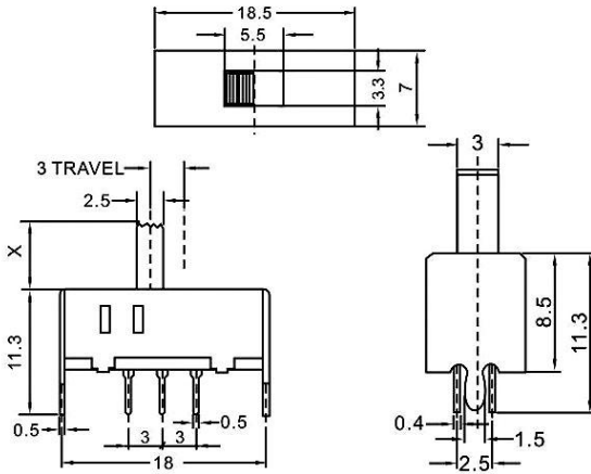
Outline Drawing
