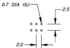
Mounting
