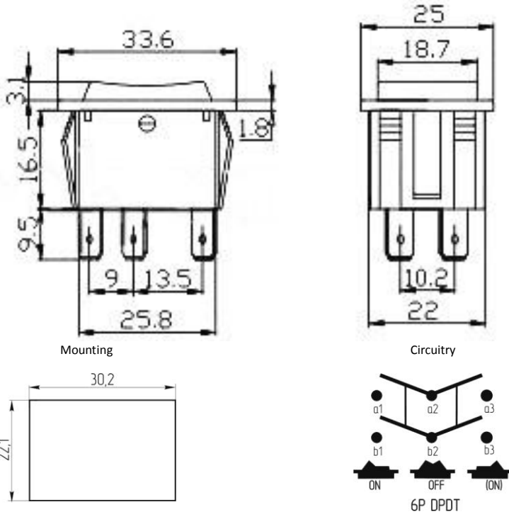
Outline Drawing
