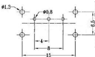
Mounting
