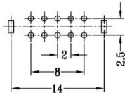
Mounting
