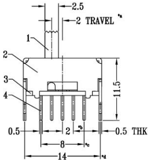
Mounting
