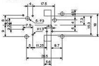
Mounting
