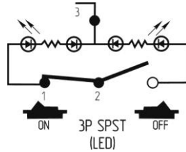
Circuitry
