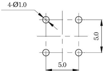
Mounting
