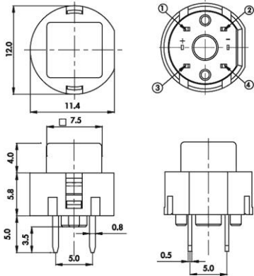
Mounting
