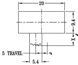
Outline Drawing
