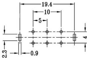
Mounting
