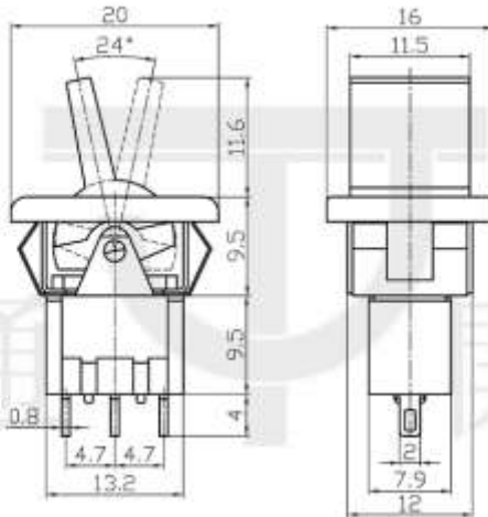
Outline Drawing
