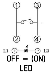
Circuitry
