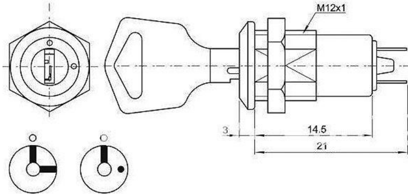
Mounting
