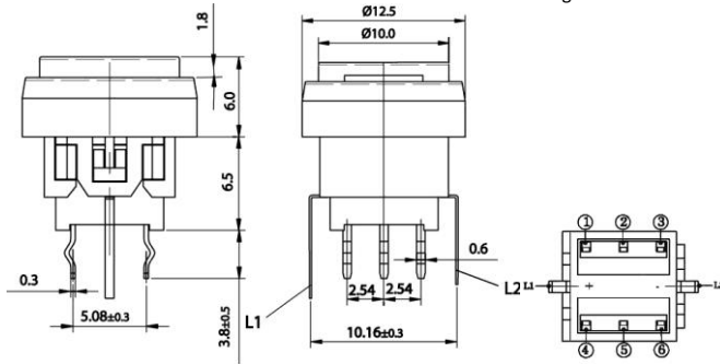
Outline Drawing
