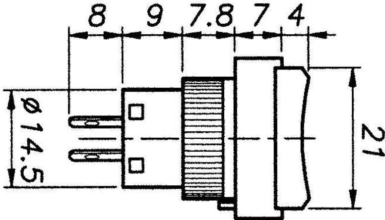
Outline Drawing
