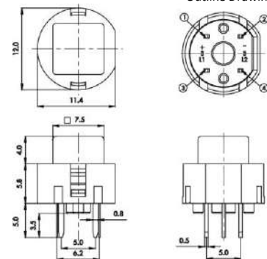
Outline Drawing
