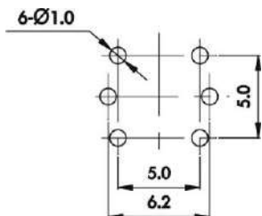
Mounting
