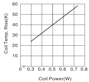
Coil Temp. Rise
