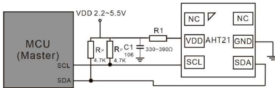
Figure 16. Typical application circuit
