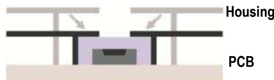
Figure 13. Small measurement dead zone helps the sensor to quickly and comprehensively detect environmental changes.
