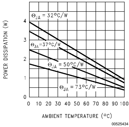
Maximum Power Dissipation (TO-263) (Note 4)
