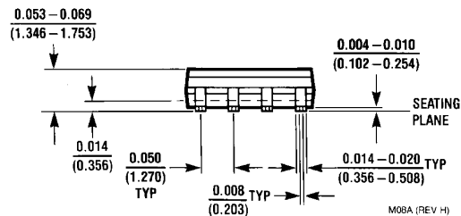
8-Lead Surface Mount Package (M) NS Package Number M08A
