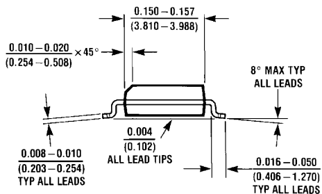
8-Lead Surface Mount Package (M) NS Package Number M08A
