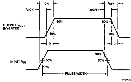
Figure 12 Switching Waveforms
