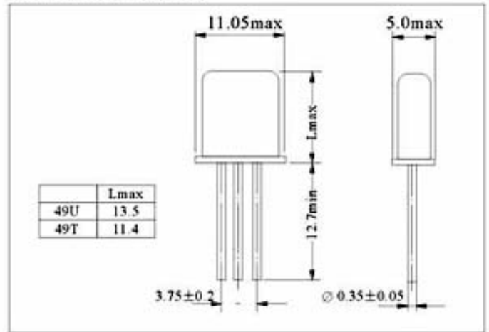
DIMENSIONS(mm)外形尺寸
