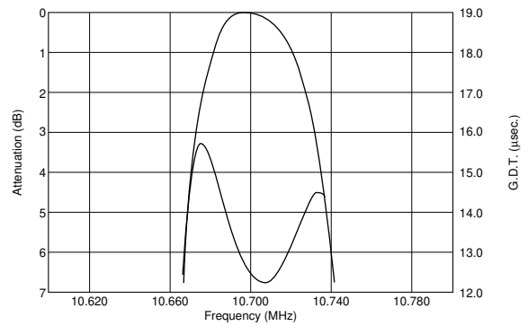
SFVLA10M7MF00-B0
