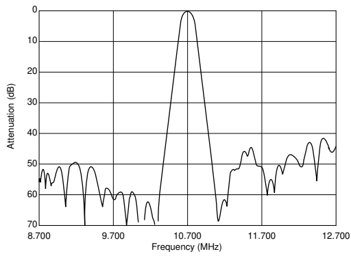
SFELB10M7HA00-B0
