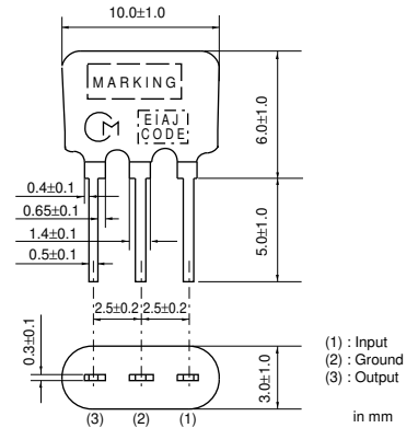
SFTLA10M7HA00-B0
