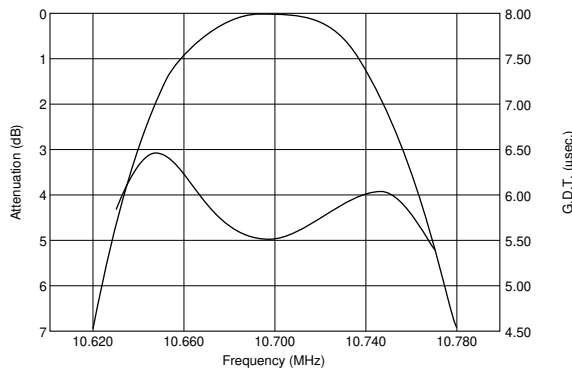
SFELA10M7KAH0-B0
