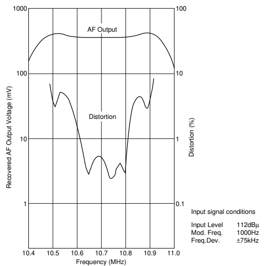
Frequency Characteristics
