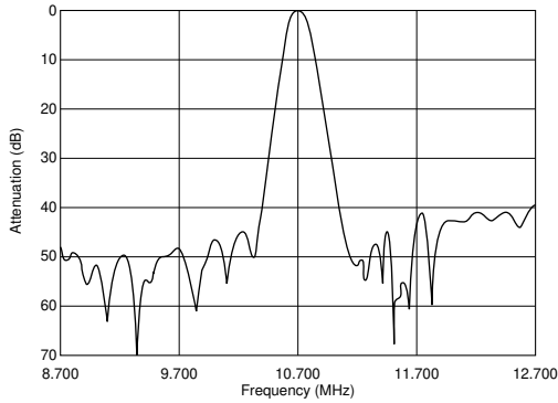
SFELA10M7JAXE-B0
