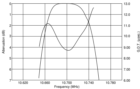
SFVLA10M7LF00-B0
