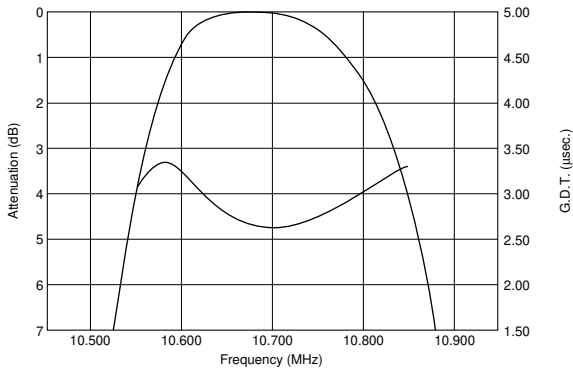
SFELA10M7FA00-B0
