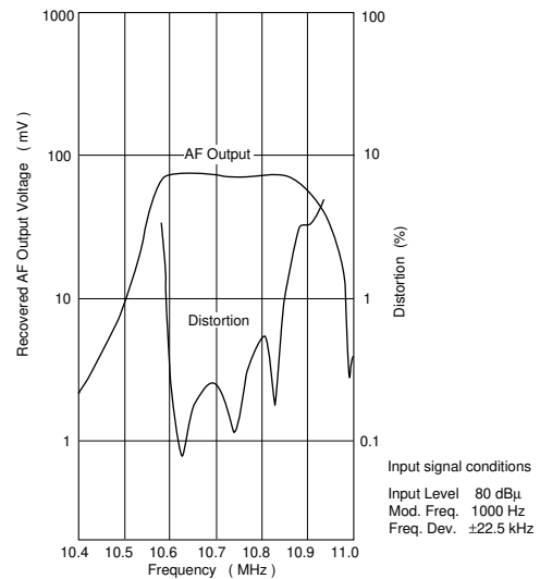
Frequency Characteristics
