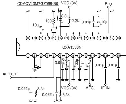
Test Circuit
