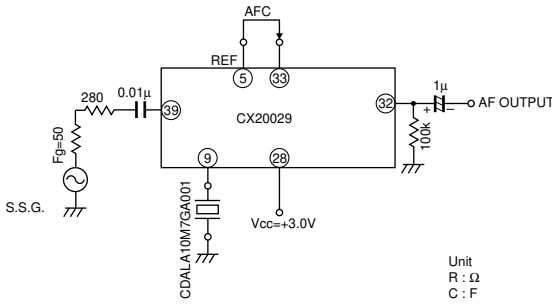
Test Circuit
