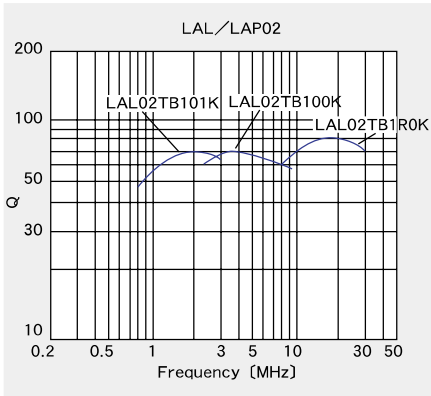
Q- 数特性例 Q-Characteristics(Measured by HP4342A)
