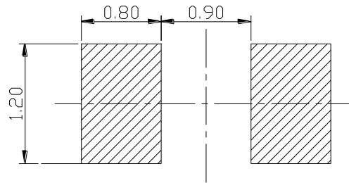
推荐焊盘尺寸 Recommended Soldering Pad
