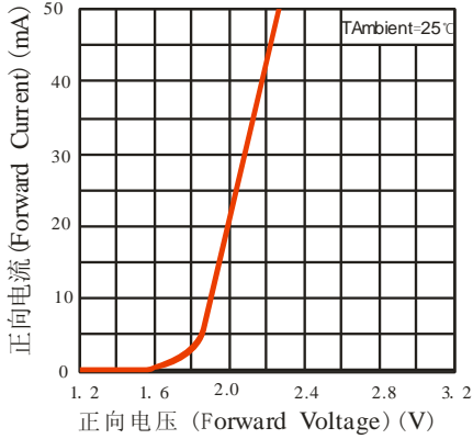
Volt-Ampere Characteristics
