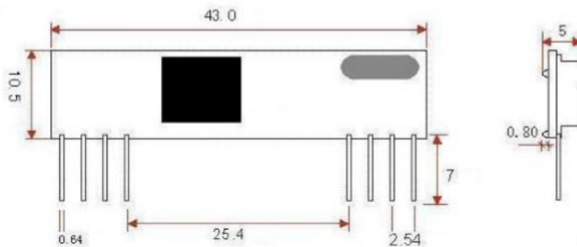
Figure2 CY01 Dimension
