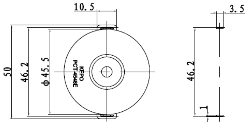
PCB FOOTPRINT
