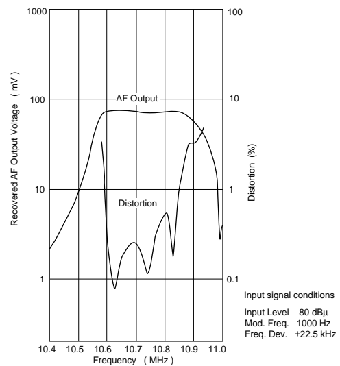
Frequency Characteristics
