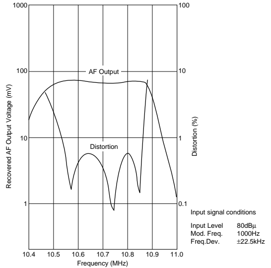
Frequency Characteristics
