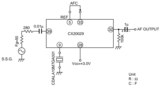
Test Circuit
