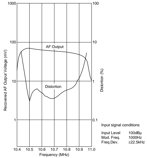
Frequency Characteristics
