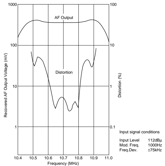
Frequency Characteristics
