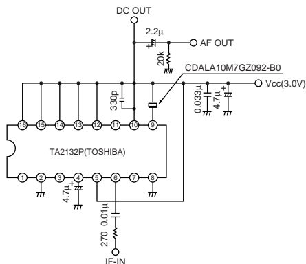
Test Circuit
