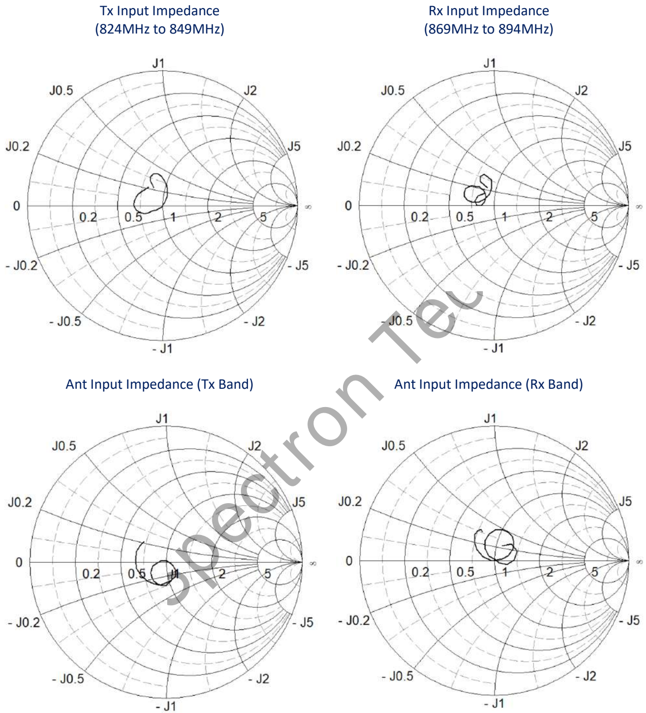
Figure 7 Input Impedances.
