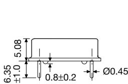
Figure 1) T Series – Side and Bottom views
